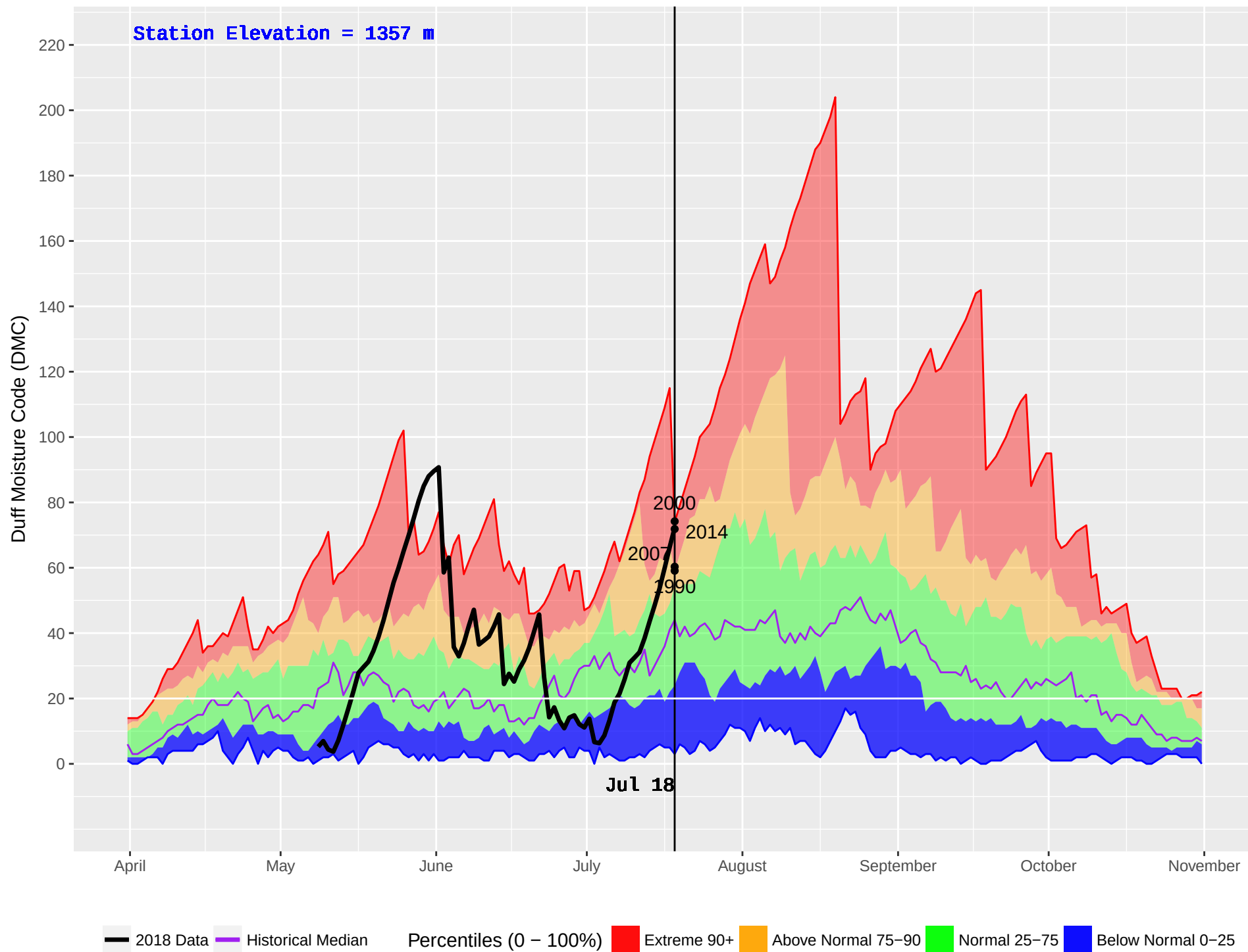
WHITE RIVER (790) : Historical (1989–2016) and Current (2018) Daily Duff Moisture Code (DMC)
