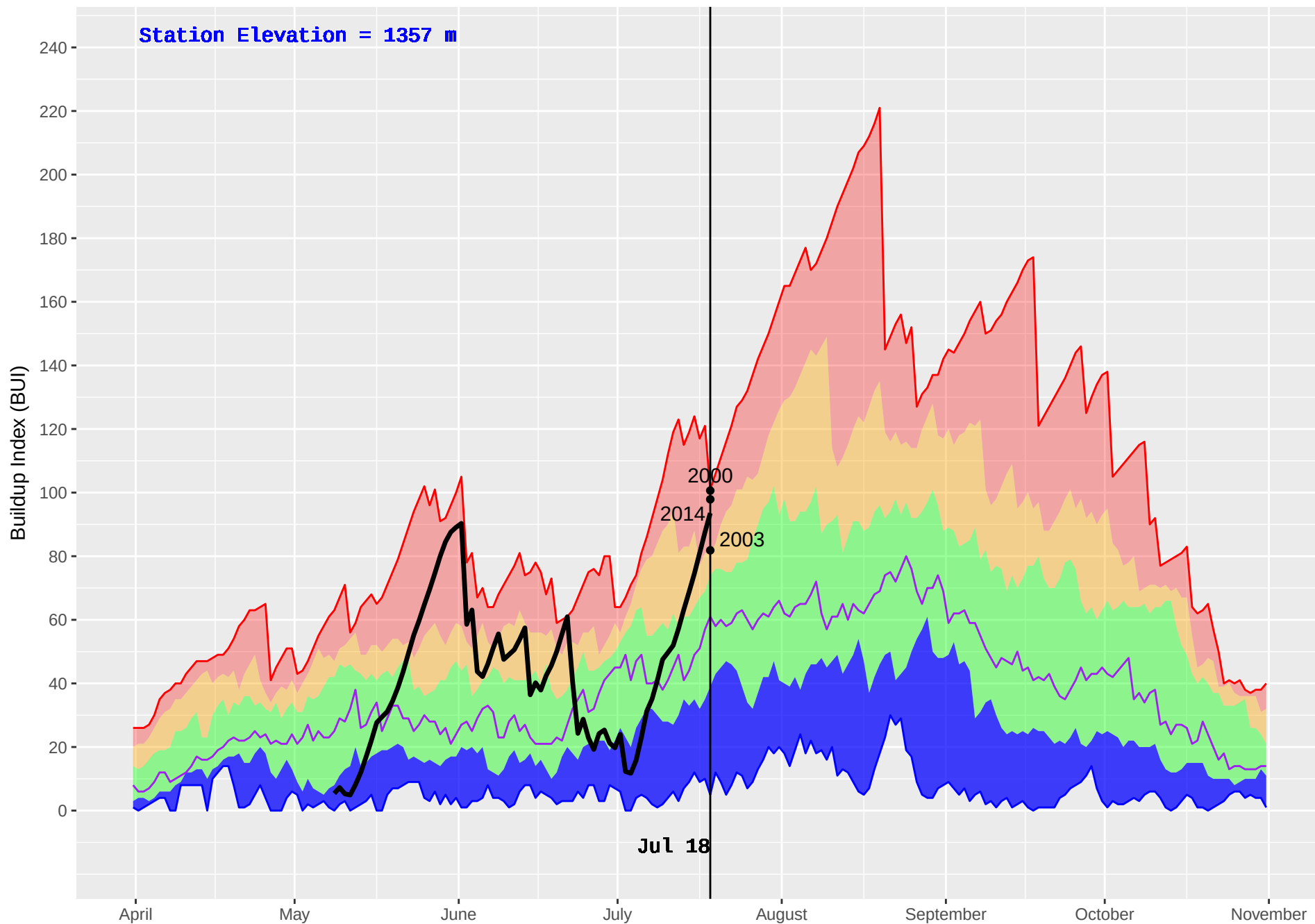
WHITE RIVER (790) : Historical (1989–2016) and Current (2018) Daily Buildup Index (BUI)
