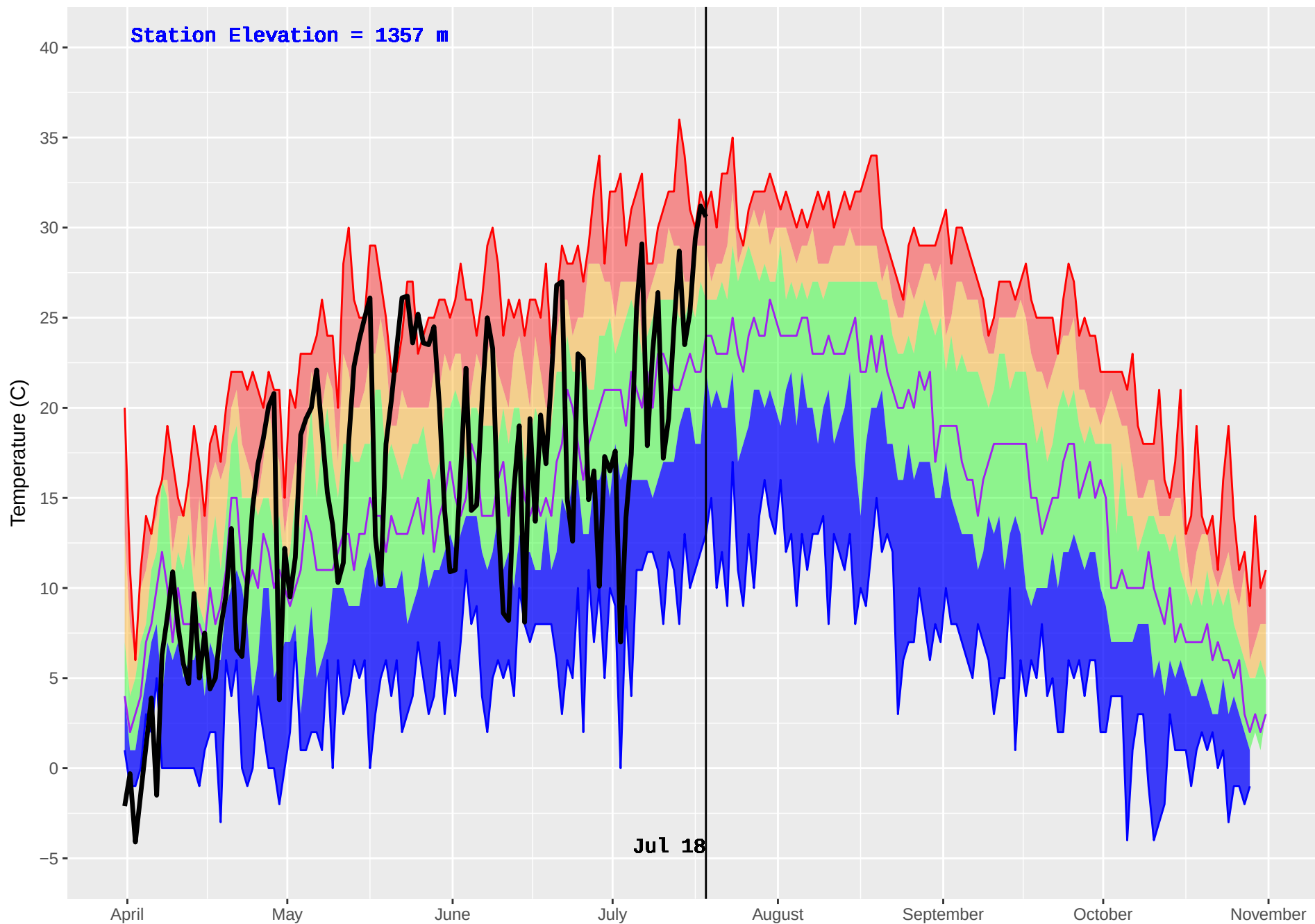
WHITE RIVER (790) : Historical (1989–2016) and Current (2018) Daily Temperature
